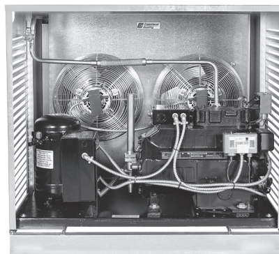
Condensing Unit
