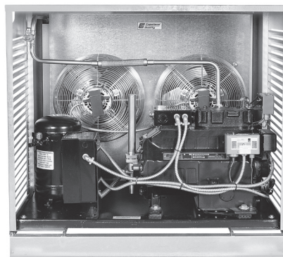
Condensing Unit
